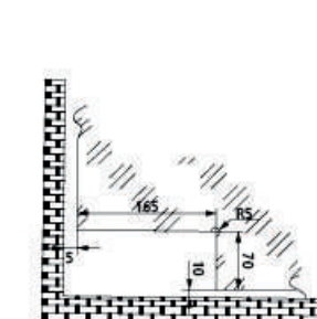
Product dimension
