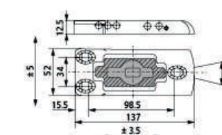
Base dimension
