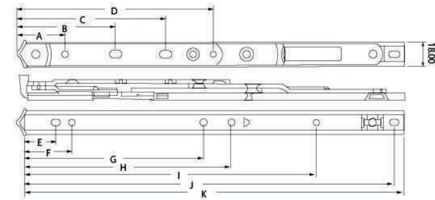
Quality Stainless Steel Slide Pallet with PVC Coating
