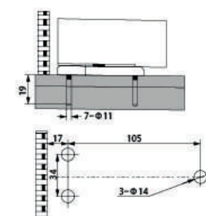
Product dimension
