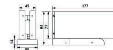
Product dimension
